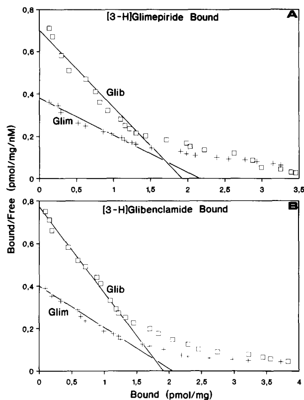
Fig. 11. Competitive Scatchard plot analysis of [ ^3 H]glimepiride (Panel A) and [ ^3 H]glibenclamide (Panel B) binding to solubilized RINm5F cell membrane proteins by glimepiride and glibenclamide. The experiments were carried out as described in the legend to Fig. 1 but using 200 \mu g of digitonin-solubilized RINm5F cell membrane proteins and precipitation of the solubilized proteins with poly(ethylene glycol) prior to filtration.
