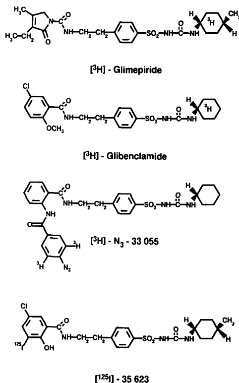
Fig. 2. Chemical structure of [ ^3\text{H} ]glimepiride, [ ^3\text{H} ]glibenclamide, \text{N}_3 -[ ^3\text{H} ]33055 and [ ^{125}\text{I} ]35623.
