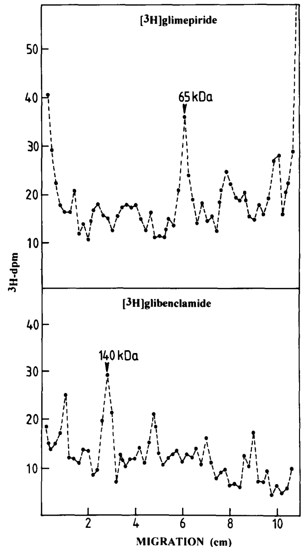
Fig. 7. Photoaffinity labeling of RINm5F cells with [ ^3 H]glimepiride and [ ^3 H]glibenclamide. RINm5F cells ( 1 \cdot 10^6 cells/ml) were incubated (10 min, 20°C) with 25.6 nM [ ^3 H]glimepiride (0.5 \mu Ci) or 25.4 nM [ ^3 H]glibenclamide (0.5 \mu Ci) in the dark and subsequently irradiated at 254 nm for 2 min. After washing, the particulate material was collected by centrifugation, suspended, precipitated and finally proteins were separated by SDS-PAGE. The distribution of ^3 H radioactivity as determined by liquid scintillation counting of the sliced gels.
