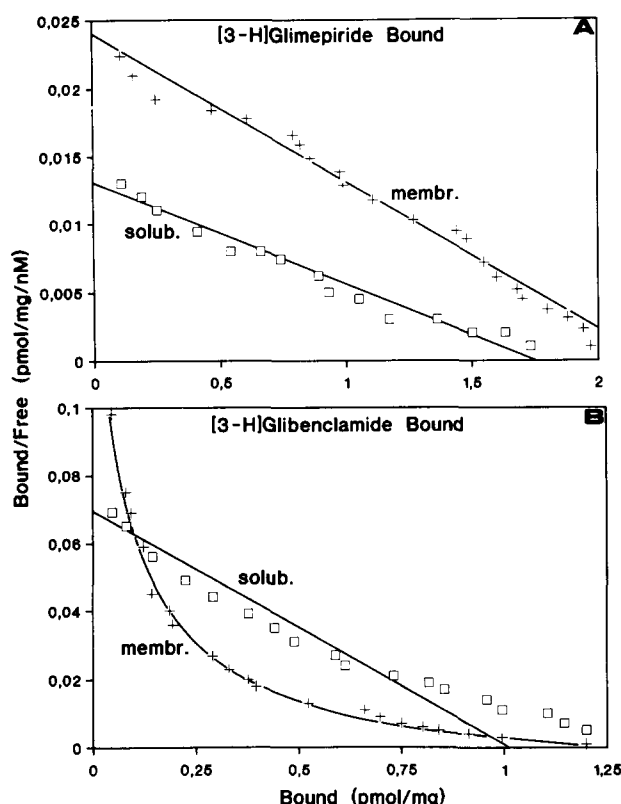
Fig. 12. Competitive Scatchard plot analysis of [ ^3\text{H} ]glimepiride (Panel A) and [ ^3\text{H} ]glibenclamide (Panel B) binding by iodo-35623. The experiments were carried out as described in the legends to Figs. 1 and 11 by incubation (60 min, 25°C) of 200 \mu\text{g} of RINm5F cell membranes (+, membr.) and digitonin-solubilized RINm5F cell membrane proteins ( \square , solub.) in the presence of 1 nM–10 \mu\text{M} unlabeled iodo-35623 and then (after precipitation of the solubilized proteins with poly(ethylene glycol)) rapidly filtered. Specific glimepiride-binding and glibenclamide-binding was determined and the means of at least 10 independent determinations were used for Scatchard plot analysis shown in the figure.
