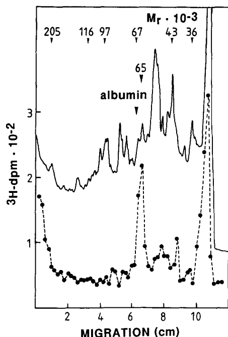
Fig. 4. Photoaffinity labeling of \beta -cell tumor membranes with [ ^3\text{H} ]glimepiride. \beta -cell tumor membranes (600 \mu\text{g} protein) were incubated (60 min, 20^\circ\text{C} ) in the dark with 30.76 nM [ ^3\text{H} ]glimepiride (0.5 \mu\text{Ci} ) and subsequently irradiated at 254 nm for 2 min. After washing of the membranes, proteins were separated by SDS-PAGE. The continuous line shows the distribution of Serva-blue R-250 stained polypeptides, the broken line denotes the distribution of ^3\text{H} radioactivity as determined by liquid scintillation counting of the sliced gels. Molecular masses (in kDa; at top of the figure) of the marker proteins are indicated by arrows.
