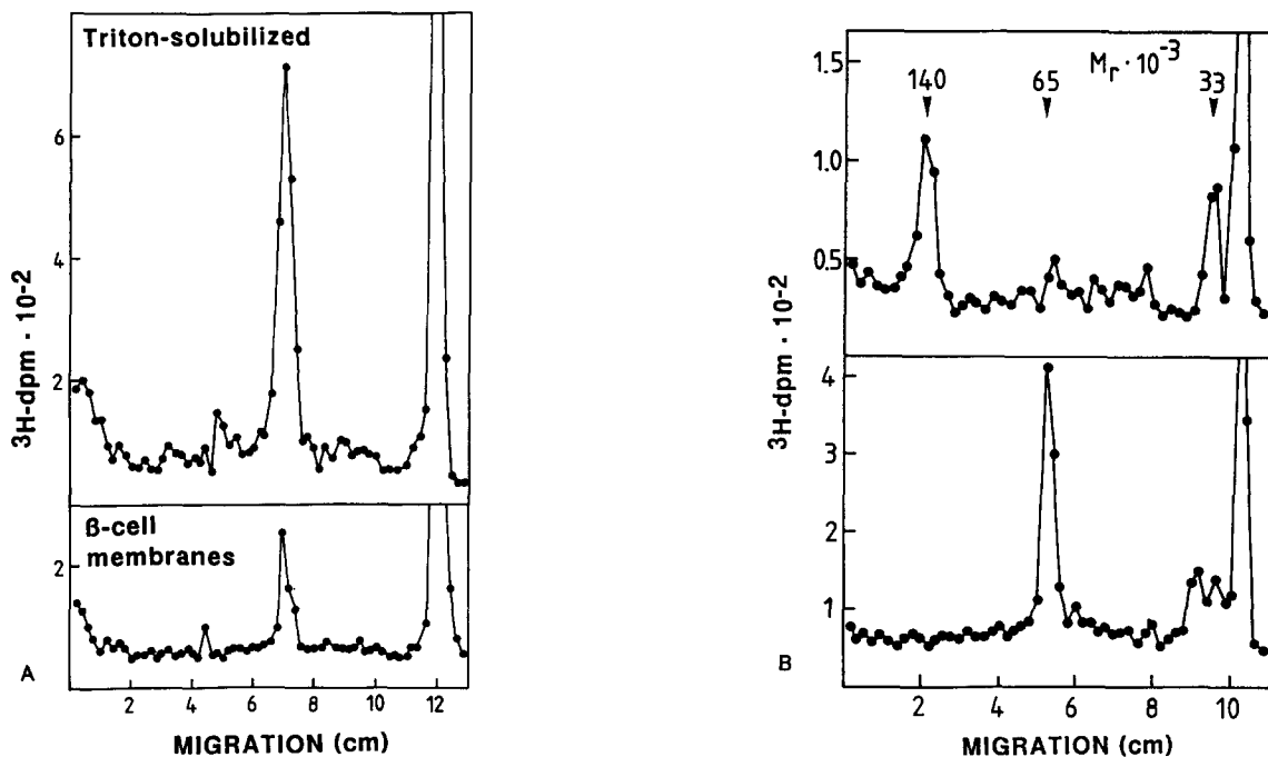
Fig. 10. Photoaffinity labeling of solubilized \beta -cell membrane proteins with [ ^3H ]glimepiride (Panel A) and [ ^3H ]glibenclamide (Panel B). \beta -cell tumor membranes and solubilized \beta -cell tumor membrane proteins (Panel A: 1% TX-100; Panel B: 1% CHAPS) (600 \mu g protein) were incubated (60 min, 20°C) with 30.76 nM [ ^3H ]glimepiride (0.5 \mu Ci) (Panel A) or 48.3 nM [ ^3H ]glibenclamide (0.3 \mu Ci) (Panel B) in the dark and subsequently irradiated at 254 nm for 2 min. After washing of the membranes, proteins were separated by SDS-PAGE. The distribution of ^3H radioactivity along the gel was determined by liquid scintillation counting of the sliced gels. The molecular weights (at top of the figure) are indicated by arrows.
