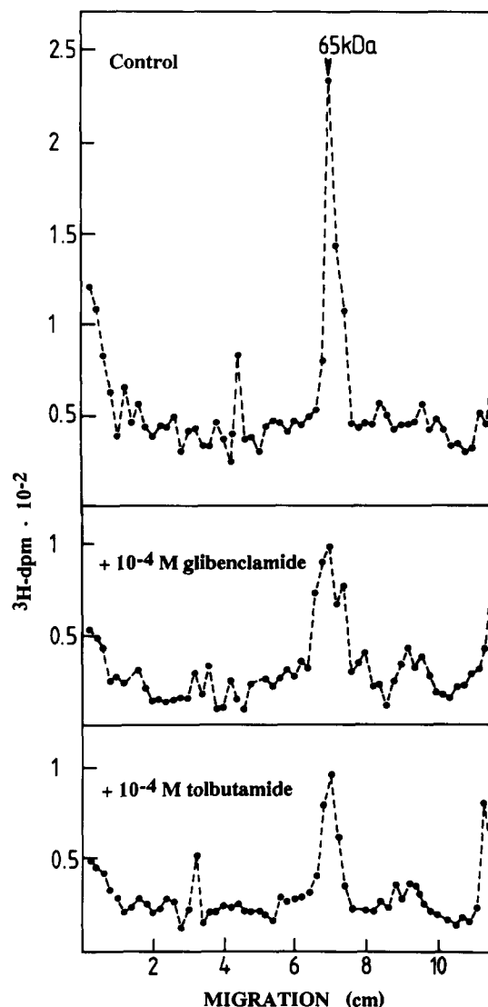
Fig. 9. Competitive photoaffinity labeling of the 65 kDa protein by glibenclamide and tolbutamide. \beta -cell tumor membranes (500 \mu g protein) were incubated (60 min, 20°C) in the dark in the absence (upper panel) or presence of 10^{-4} M glibenclamide (middle panel) or 10^{-4} M tolbutamide (lower panel). After incubation (10 min, 20°C) with 30.76 nM [ ^3 H]glimepiride (0.5 \mu Ci) in the dark, the membranes were irradiated at 254 nm for 2 min. After washing of the membranes, proteins were separated by SDS-PAGE and counted for radioactivity by liquid scintillation counting of the sliced gels.
