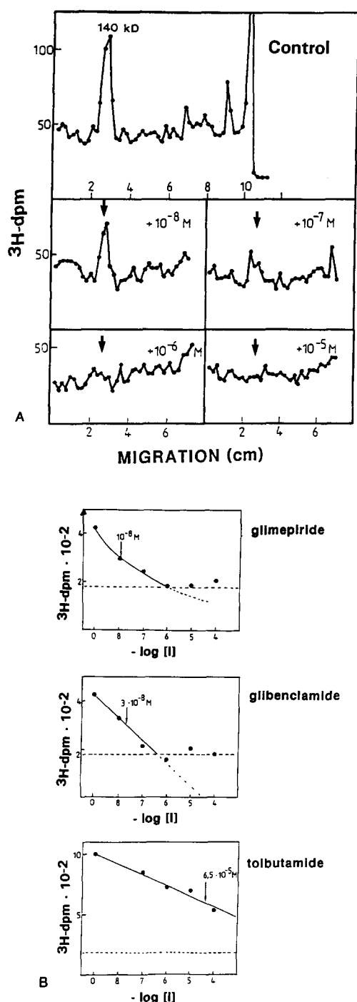
Fig. 8. Competitive photoaffinity labeling of the 140 kDa protein by glimepiride, glibenclamide and tolbutamide. \beta -cell tumor membranes (600 \mu g protein) were incubated (60 min, 20°C) in the dark in the presence of various concentrations ( 10^{-8} to 10^{-4} M) of glimepiride, glibenclamide or tolbutamide. After incubation (10 min, 20°C) with 60 nM [ ^3 H]glibenclamide (0.37 \mu Ci) in the dark, the membranes were irradiated at 254 nm for 2 min. After washing of the membranes, the proteins were separated by SDS-PAGE and counted for radioactivity by liquid scintillation counting of the sliced gels (shown only for glimepiride in Panel A). The logarithmic plots of the drug concentration used for the competition versus the ^3 H-radio-label bound to the 140 kDa protein are shown in Panel B. The IC_{50} values for half-maximal inhibition of [ ^3 H]glimepiride binding are indicated by arrows.
