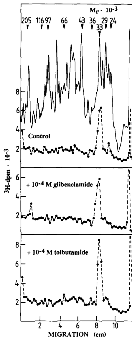
Fig. 5. Photoaffinity labeling of \beta -cell tumor membranes with \text{N}_3 -[ ^3\text{H} ]33055. \beta -cell tumor membranes (500 \mu\text{g} protein) were incubated (15 min, 20^\circ\text{C} ) and subsequently (5 min, 0^\circ\text{C} ) with 51 nM \text{N}_3 -[ ^3\text{H} ]33055 (0.65 \mu\text{Ci} ) in 100 mM sodium phosphate buffer (pH 7.4) either in the absence (upper panel) or presence of 10^{-4} M glibenclamide (middle panel) or 10^{-4} M tolbutamide (lower panel). After photolabeling at 254 nm for 30 s and washing of the membranes, proteins were separated by SDS-PAGE. The continuous line shows the distribution of Serva-blue R-250 stained polypeptides, the broken line the distribution of radioactivity.
