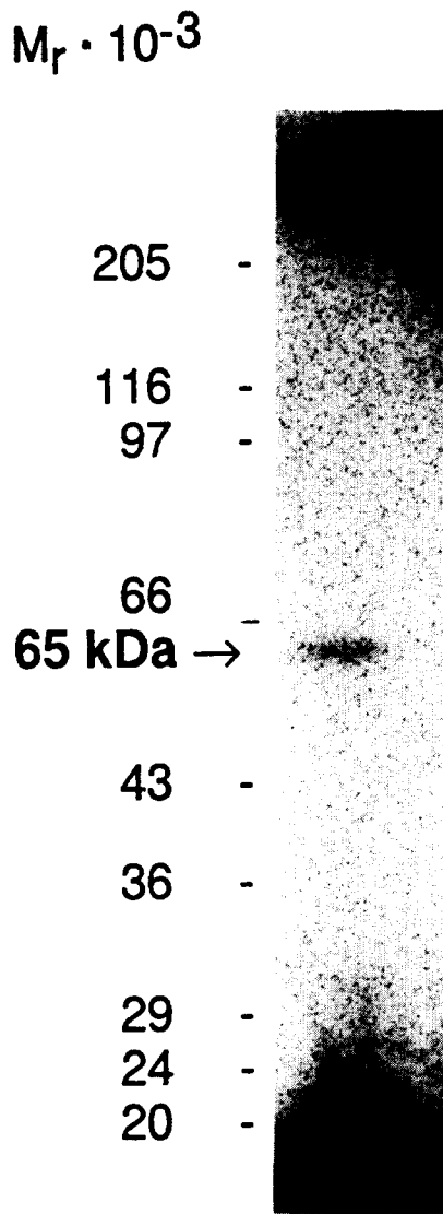
Fig. 6. Photoaffinity labeling of \beta -cell tumor membranes with [ ^{125} I]35623. \beta -cell tumor membranes (500 \mu g protein) were incubated (15 min, 20°C) with 27.6 nM [ ^{125} I]35623 (0.4 \mu Ci) in the dark and subsequently irradiated at 254 nm for 2 min. After washing of the membranes, proteins were separated by SDS-PAGE. An autoradiography of the dried gel is shown. The molecular masses indicated were derived from marker proteins run in parallel on the same gel.
