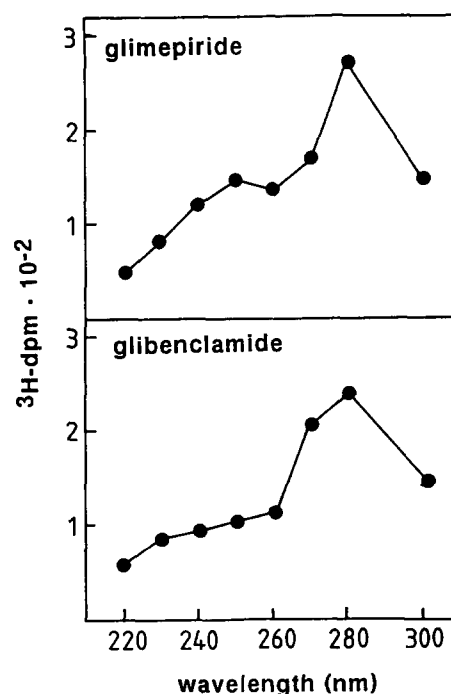
Fig. 3. Photocatalyzed incorporation of [ ^3\text{H} ]glimepiride into human serum albumin. Human serum albumin (1 mg/ml) in 100 mM sodium phosphate buffer (pH 7.4) was incubated (10 min, 20°C) with 0.25 \mu\text{M} [ ^3\text{H} ]glimepiride (8 \mu\text{Ci}/\text{mg} protein) in the dark. Photoaffinity labeling was carried out at various wavelengths between 220 and 300 nm. After 3 min irradiation, aliquots containing 40 \mu\text{g} protein were removed and protein was precipitated. The covalent attachment of [ ^3\text{H} ]sulfonylureas to albumin was determined by scintillation counting after SDS-PAGE and slicing of the gels.
