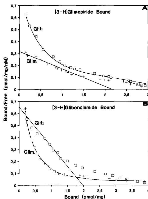
Fig. 1. Competitive Scatchard plot analysis of specific [ ^3\text{H} ]glimepiride or [ ^3\text{H} ]glibenclamide binding. 200\ \mu\text{g} of RINm5F cell membranes were incubated (60 min, 20^\circ ) with 0.5\ \text{nM} [ ^3\text{H} ]glimepiride (Panel A) or [ ^3\text{H} ]glibenclamide (Panel B) in the presence of 0.1 – 100\ \text{nM} unlabeled glimepiride (+) or glibenclamide ( \square ) and then rapidly filtered. Specific glimepiride-binding and glibenclamide-binding was determined and the means of at least 16 independent determinations obtained with four different membrane preparations were used for the Scatchard plot analysis.
